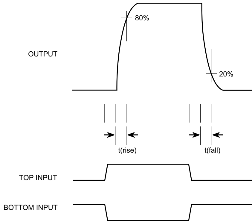
Figure 20: Output Response
