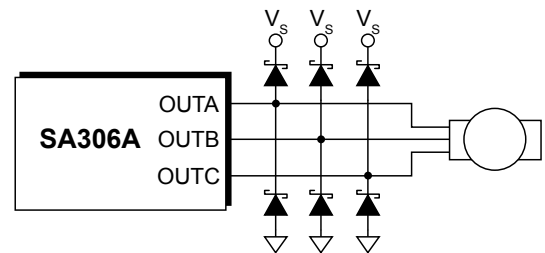
Figure 9. Schottky Diodes
