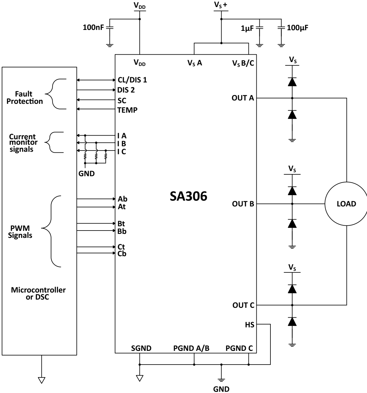
Figure 1: Typical Connection
