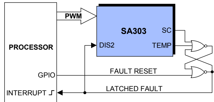
Figure 6. External Fault Latch Circuit
