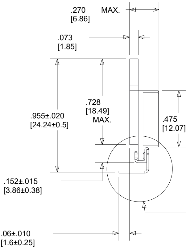
DETAIL A SCALE 4.000
