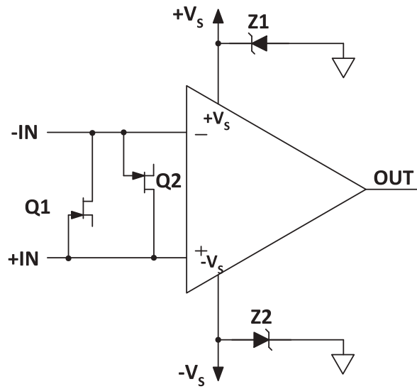
Figure 17: Overvoltage Protection
