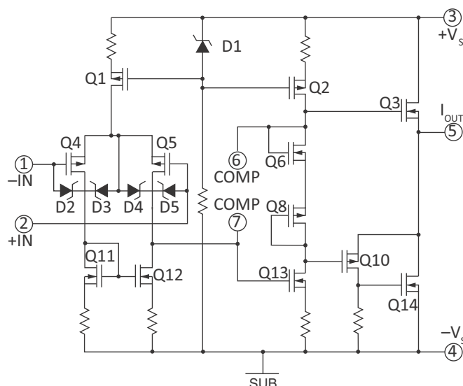
Figure 1: Equivalent Schematic
