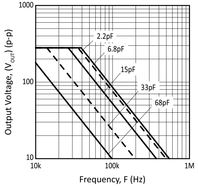
Figure 11: Slew Rate
