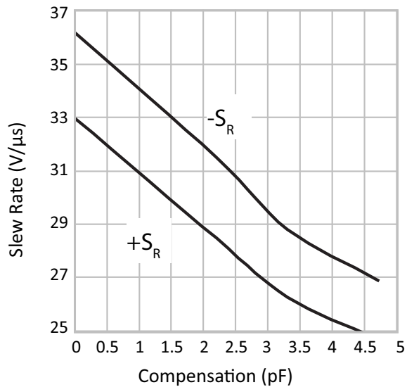
Figure 12: PA167 • PA167A Slew Rates vs. Compensation
