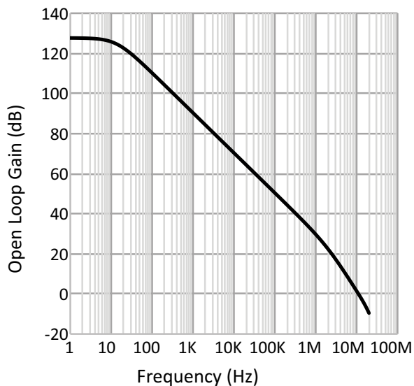
Figure 14: PA167 • PA167A Open Loop Frequency Response, C C = 0pF
