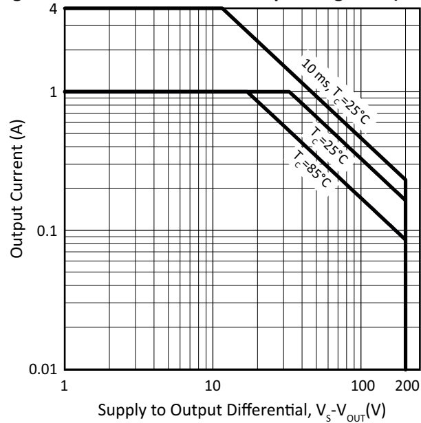
Figure 3: PA167 • PA167A Safe Operating Area (SOA)
