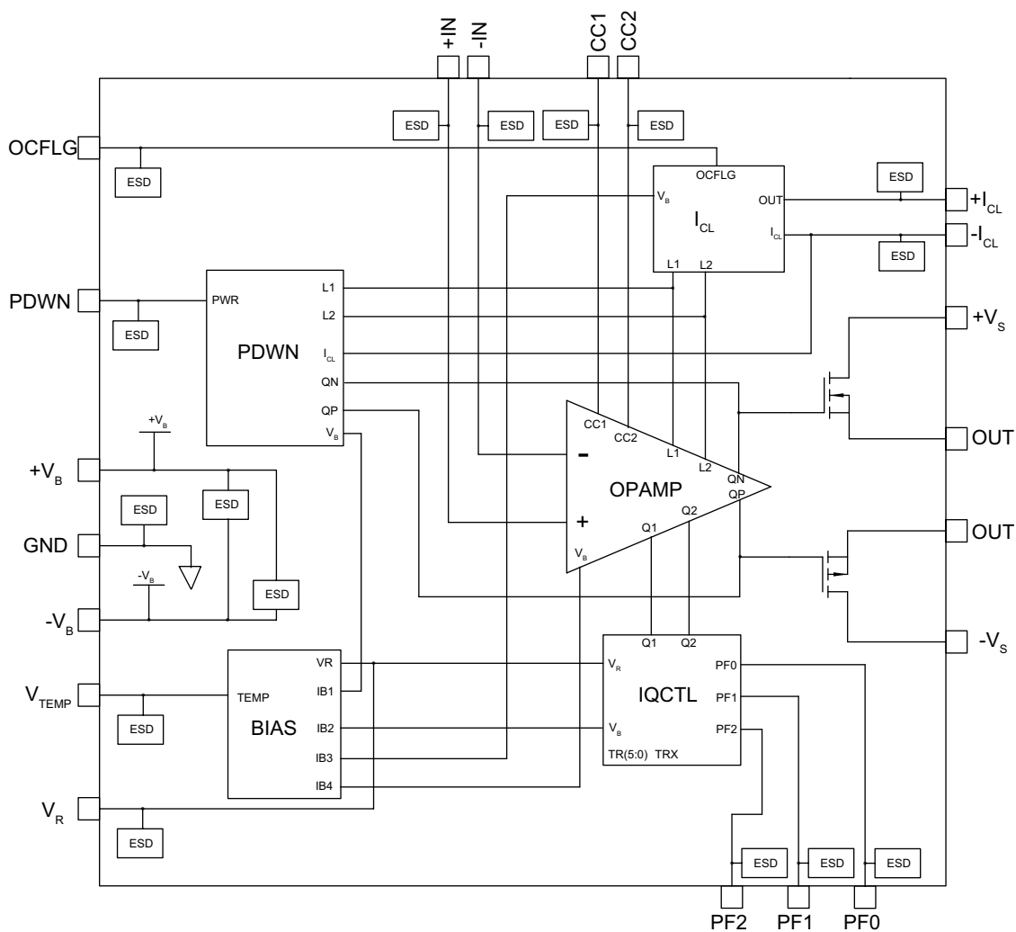
Figure 1: PA167 Block Diagram
