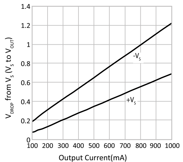
Figure 15: PA167 • PA167A Output Voltage Swing (with additional boost voltage)
