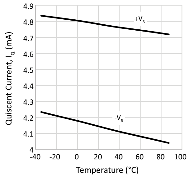
Figure 11: PA167 • PA167A V_B Quiescent Current vs. Temperature
