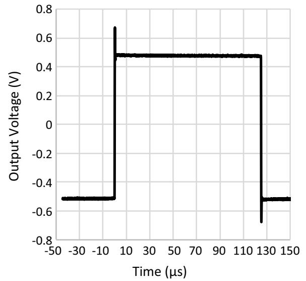
Figure 17: PA167 • PA167A Small Signal Pulse Response
