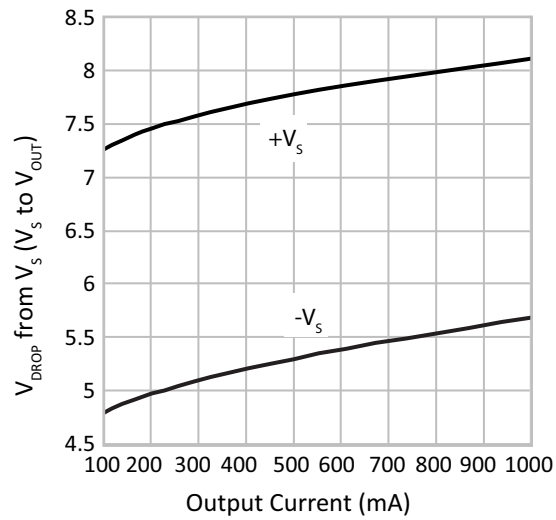
Figure 16: PA167 • PA167A Output Voltage Swing (without additional boost voltage)
