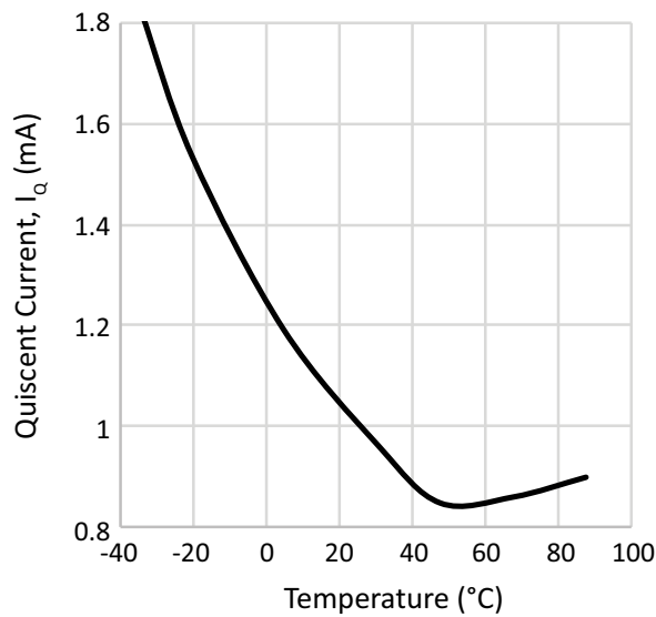
Figure 10: PA167 • PA167A V_S Quiescent Current vs. Temperature
