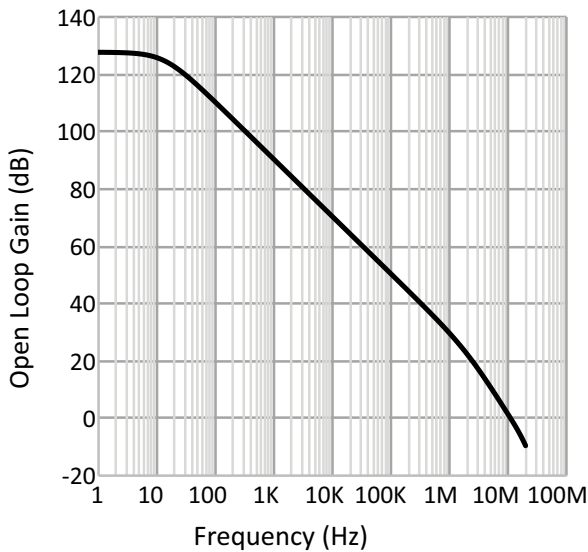
Figure 16: PA164 Open Loop Frequency Response, C_C = 0pF
