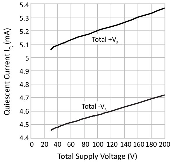
Figure 11: I_Q vs. Supply
