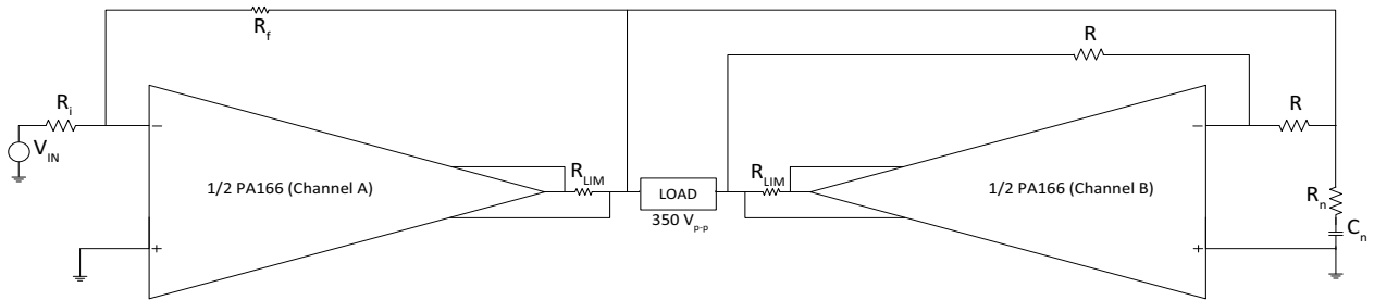
Figure 3: Bridge Configuration
