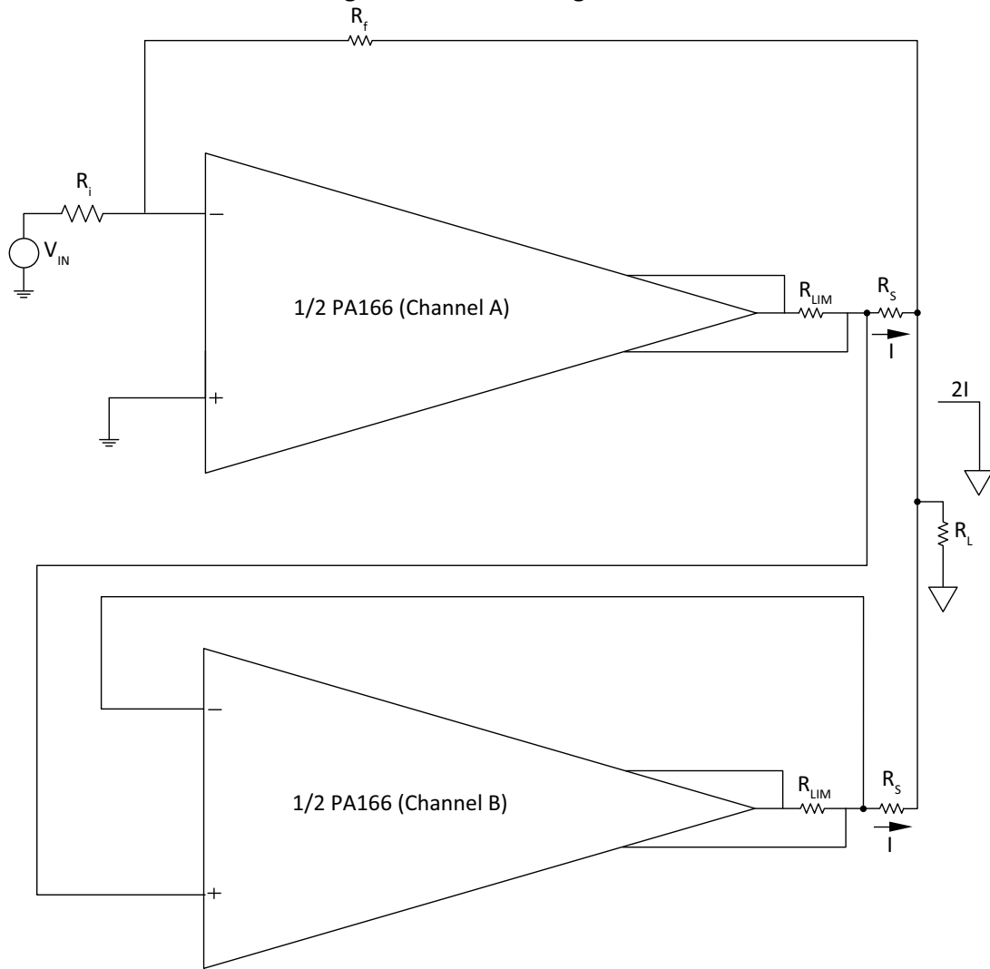
Figure 4: Parallel Configuration
