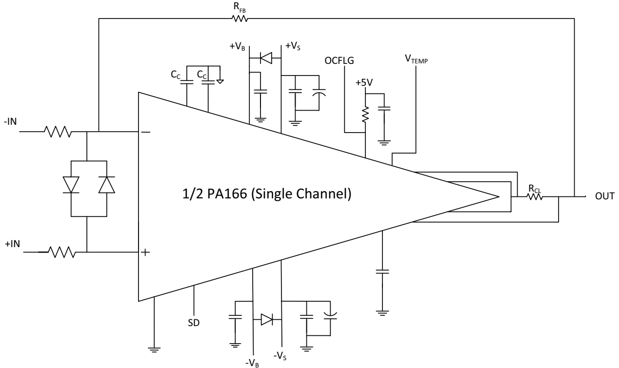
Figure 2: Typical Connection
