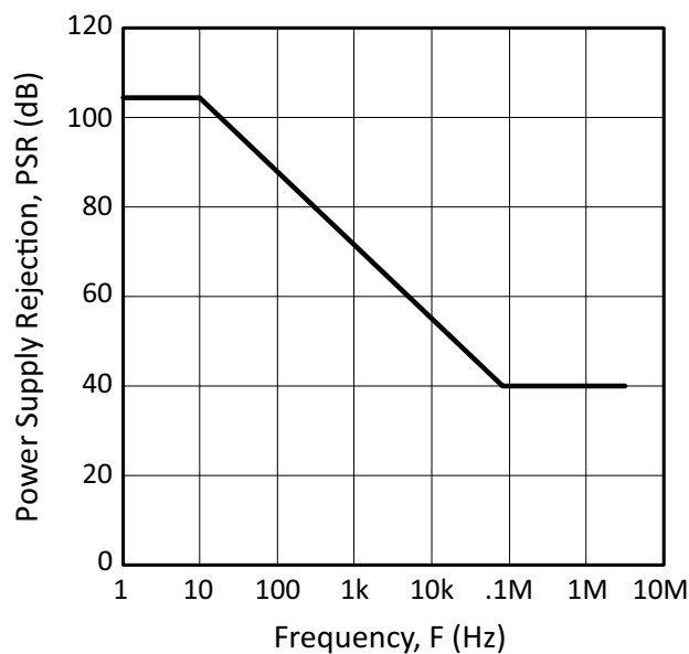
Figure 15: Power Supply Rejection
