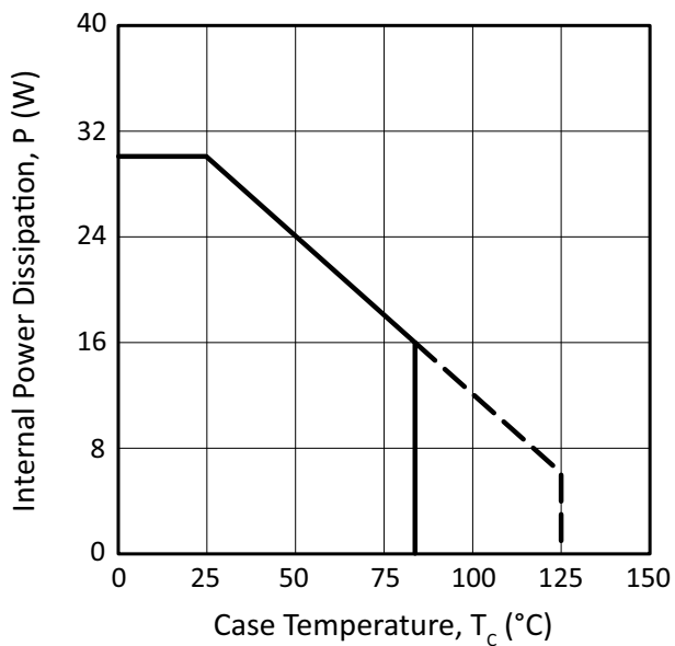
Figure 6: Power Response
