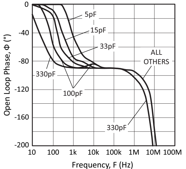
Figure 6: Phase Response
