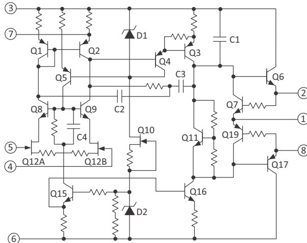
Figure 1: Equivalent Schematic
