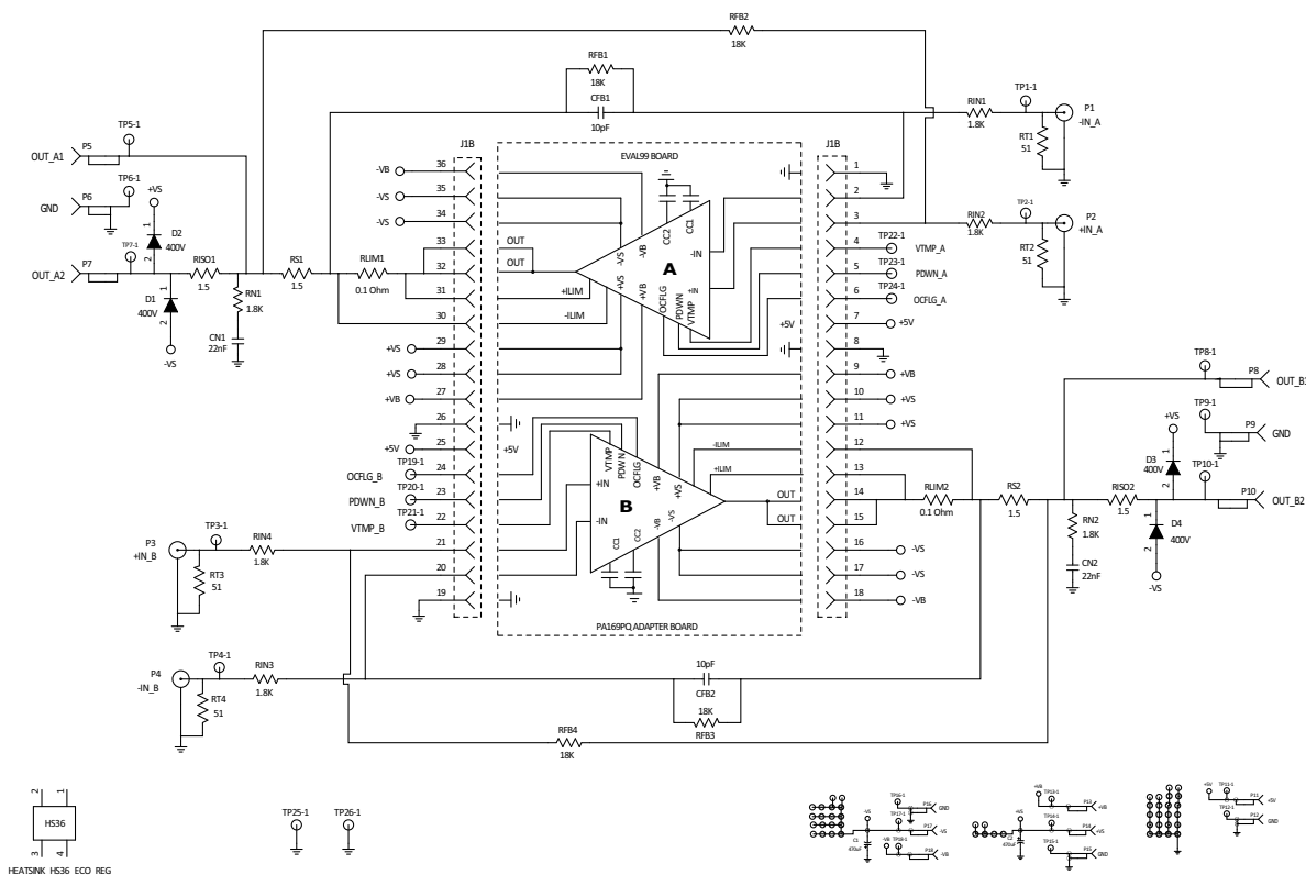
Figure 1: Circuit Diagram (Main PCB/EVAL166)
