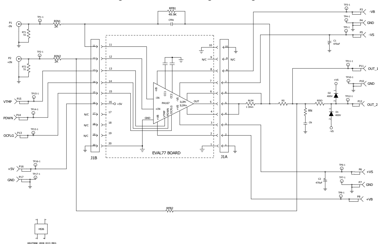
Figure 1: EK97 Circuit Configuration Diagram
