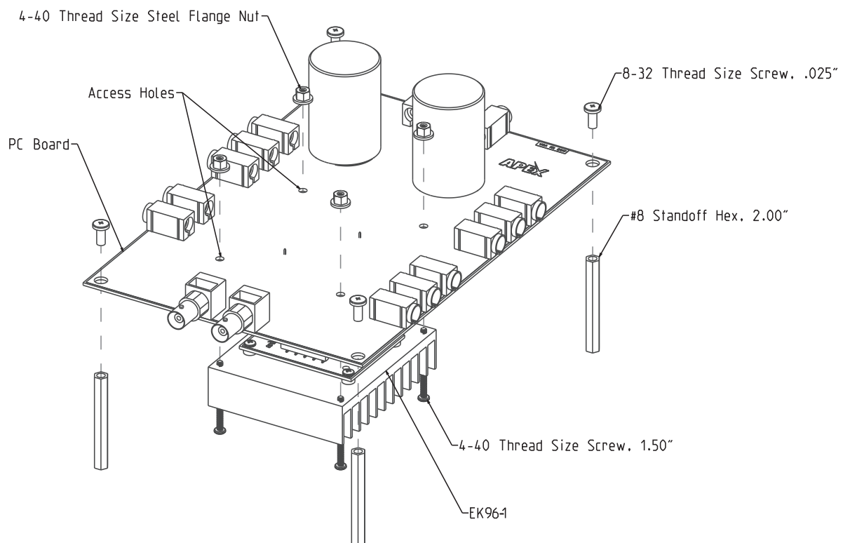
Figure 4: EK97 Build
