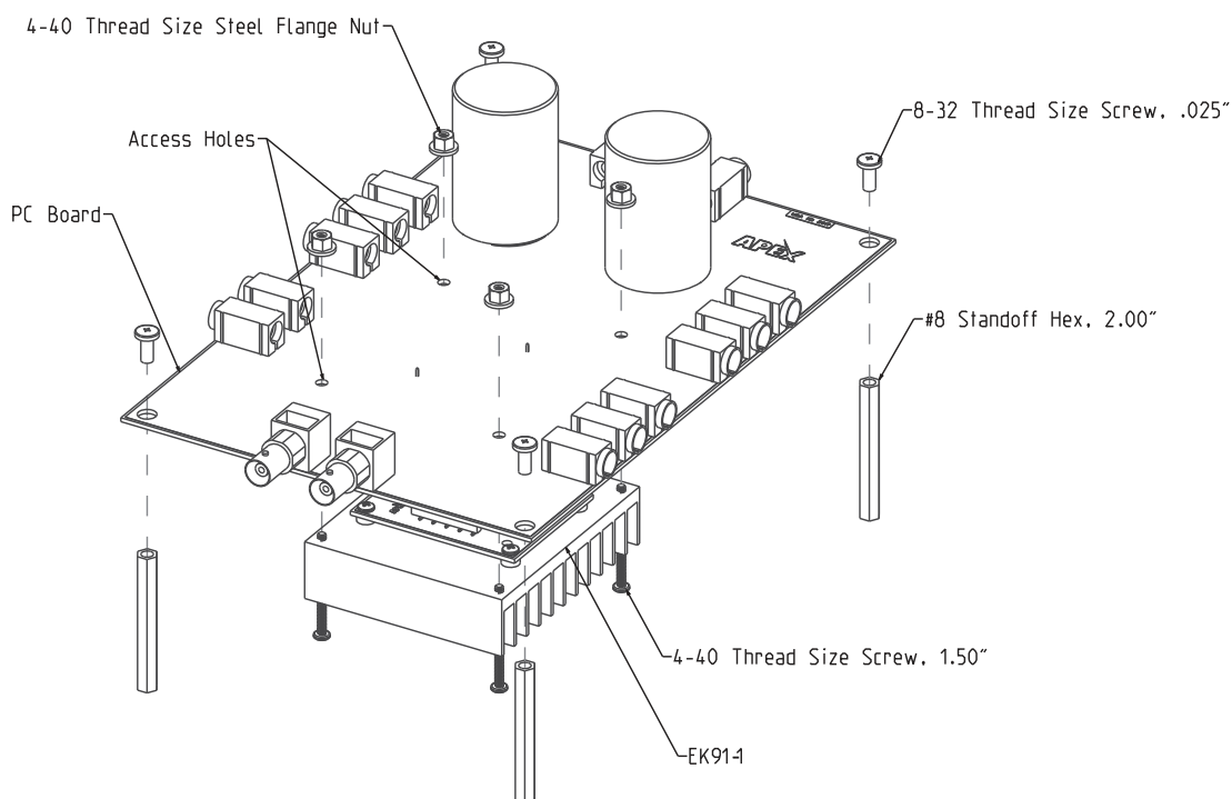
Figure 4: EK74 Build
