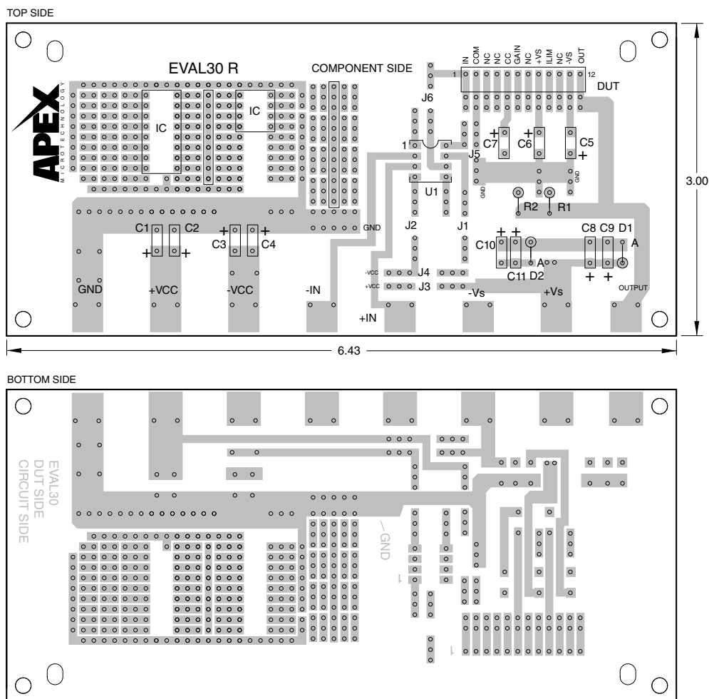
Figure 1: PCB
