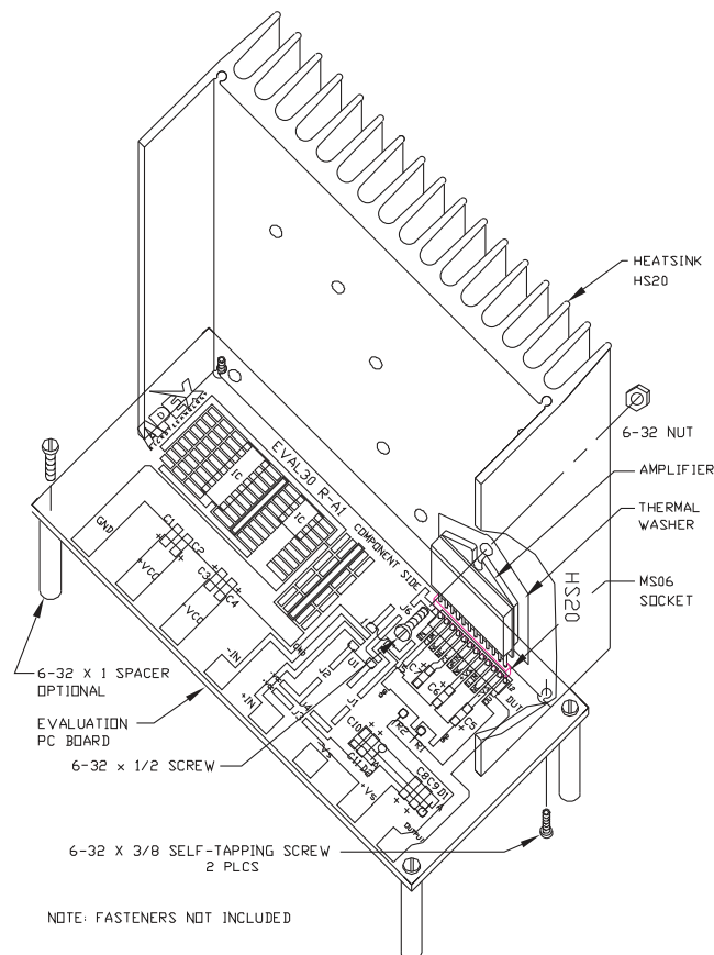
Figure 3: Assembly
