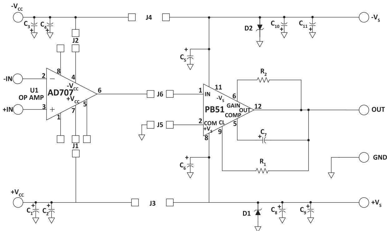
Figure 2: EK Schematic
