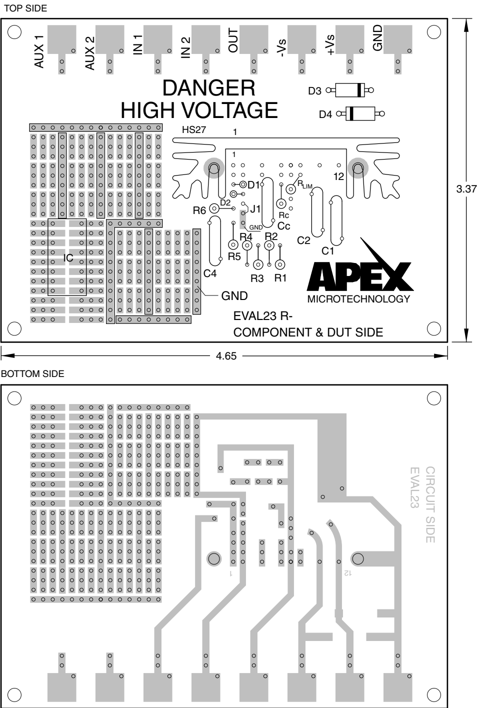
Figure 2: PCB
