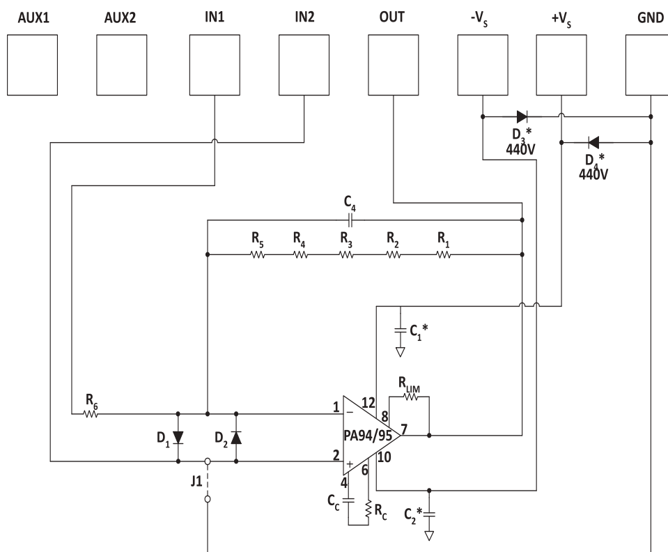
Figure 1: Schematic
