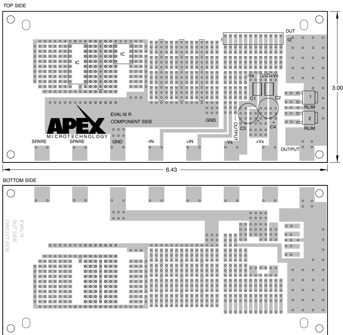
Figure 1: PCB
