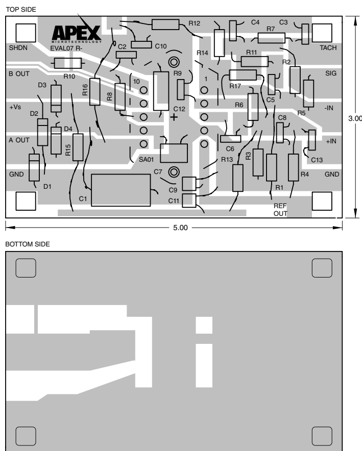
Figure 1: PCB Layout
