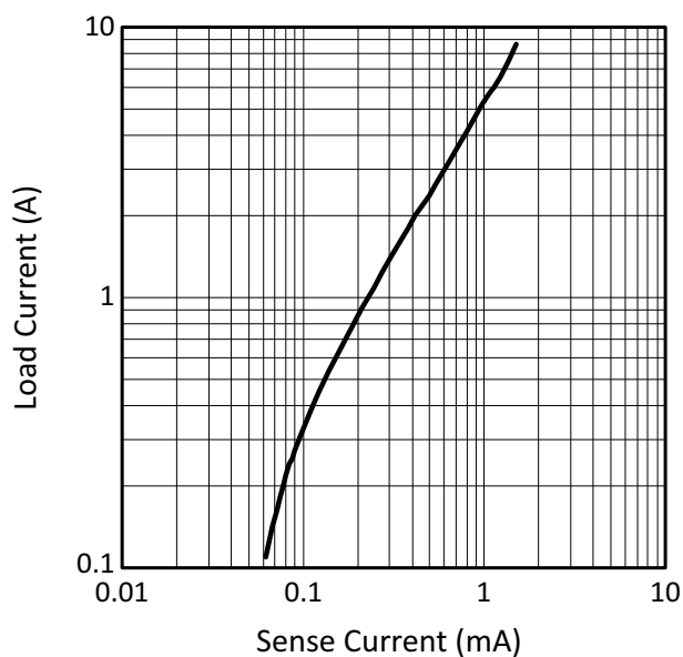
Figure 5: Current Sense
