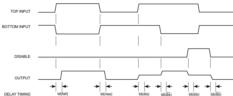
Figure 19: Timing Diagrams
