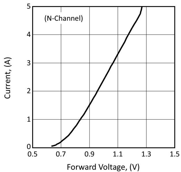
Figure 11: Diode Forward Voltage - Bottom FET
