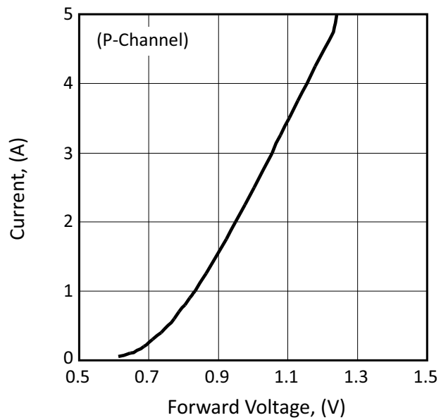
Figure 12: Diode Forward Voltage - Top FET
